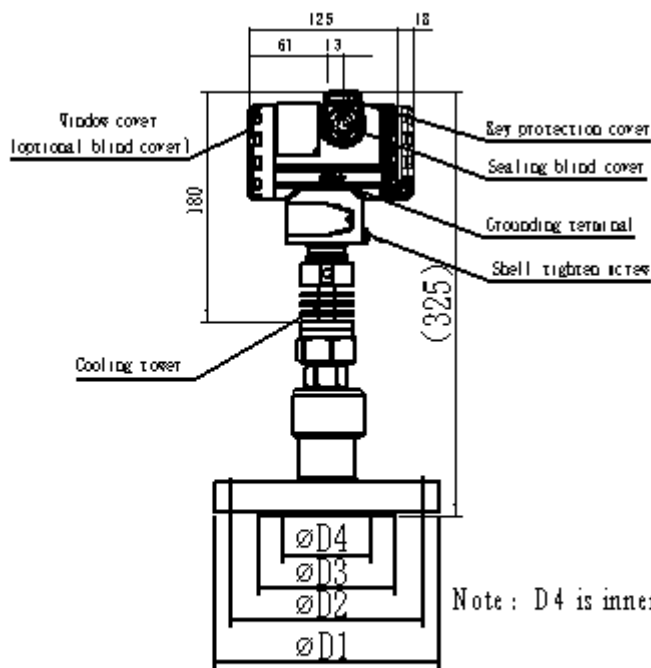
PDS879 ultrahigh temperature straight connection type
