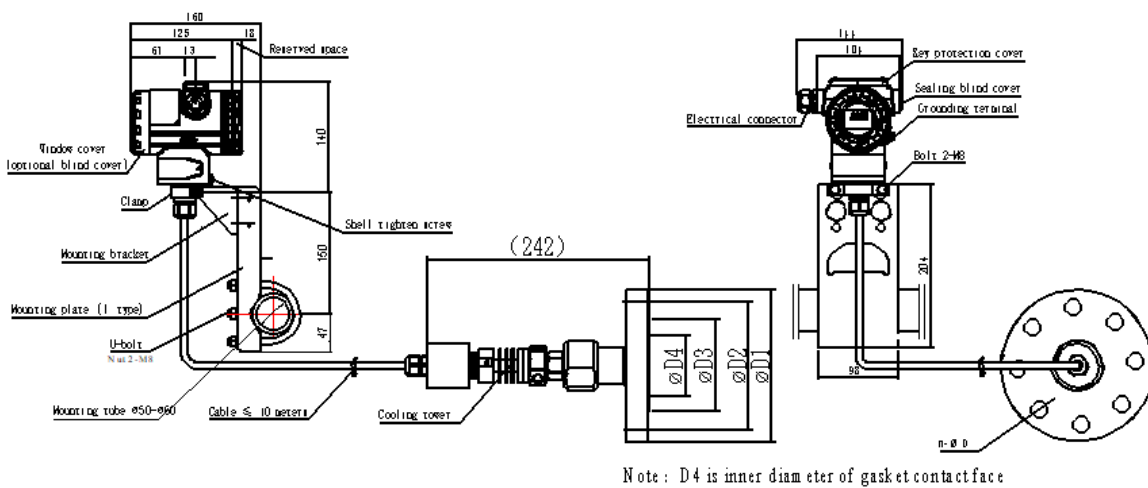
Horizontal piping mounting type (horizontal mounting tube)
